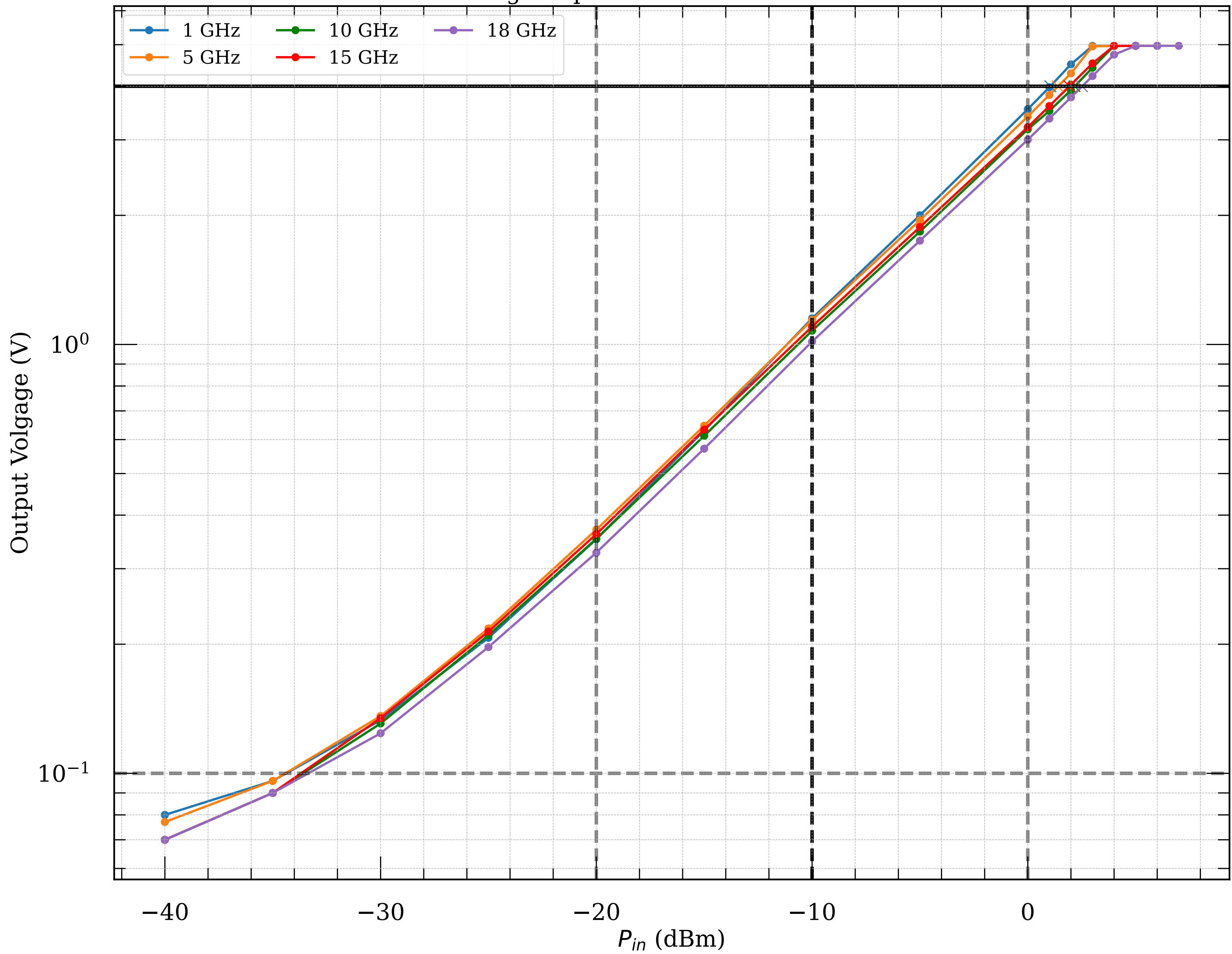
Measured voltage-to-power curve of detector module013v2
